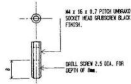
FRONT RESTRAINTING SCREW SCALE 2:1
