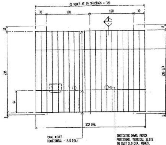
ELEVATION - WIRE CAGING NOTE: CASE WIRES - 2.0 DIA. / 2.5 DIA. TO BE CHROMIUM PLATED IN ACCORDANCE WITH SHOWCASE SPECIFICATION.
